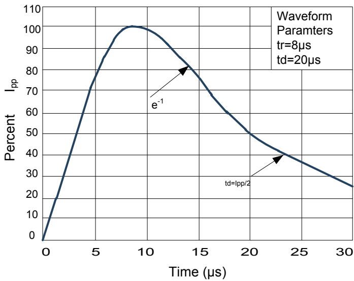
Figure3: Pulse Waveform
