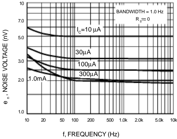
Figure 1. Noise Voltage
