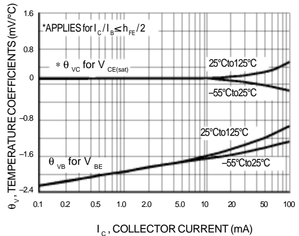
Figure 11. Temperature Coefficients
