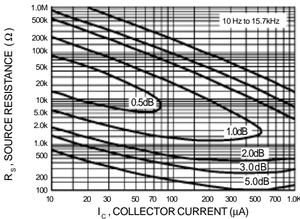
Figure 5. Wideband
