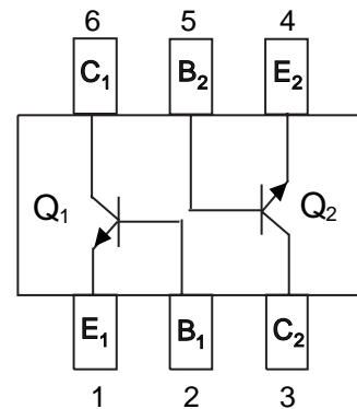
SOT-363/SC-88
